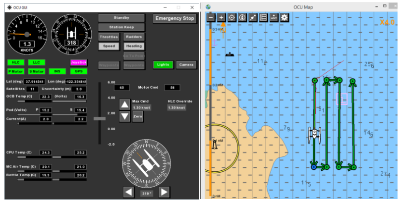
WAM-V Graphical User Interface (GUI)
